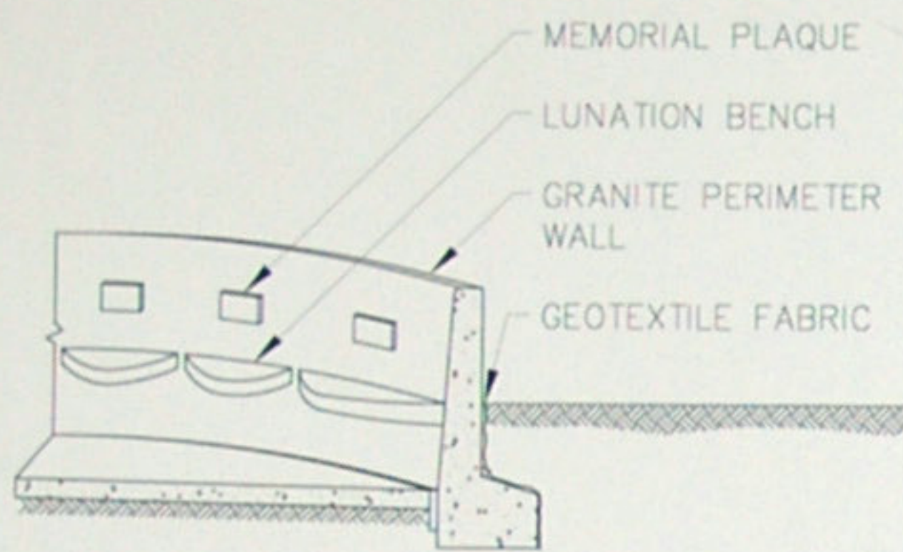
Detail 2 - Lunation Memorial Benches
